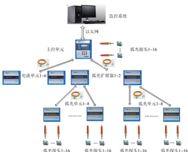
Busbar Protection System Configuration Plan
