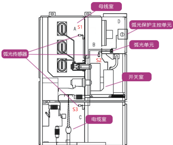
EXAMPLE OF SWITCHGEAR INTERNAL FAULT PROTECTION LOGIC
