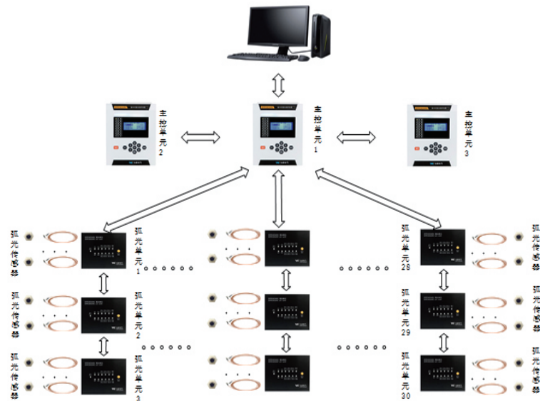
Typical Application Diagram for Fast Protection of Internal Switchgear Faults
