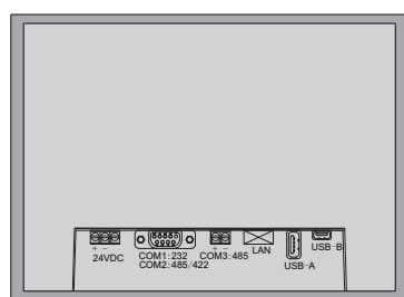
Centralized Control Panel Backplane Terminal Physical Diagram
