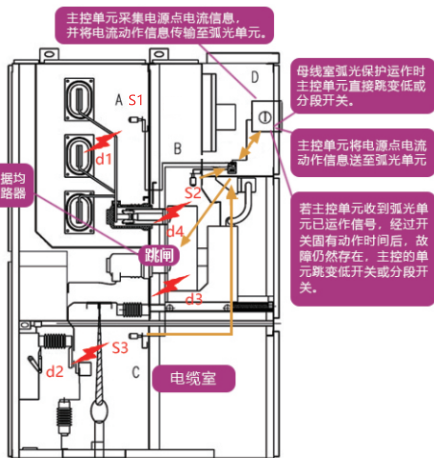
TYPICAL APPLICATION DIAGRAM FOR RAPID SWITCHGEAR INTERNAL FAULT PROTECTION
