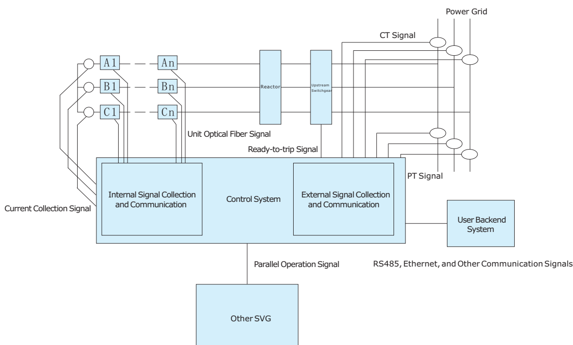
LSHSVG Star Connection Structure Diagram
