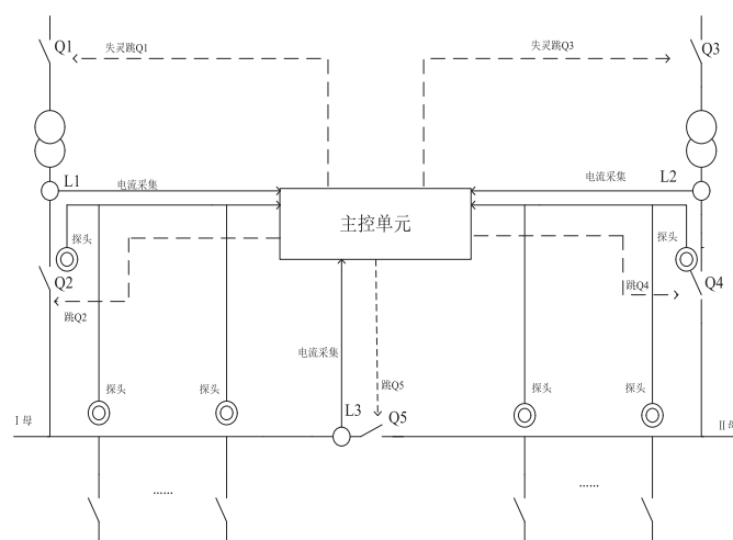
Typical Application Example of Busbar Protection System
